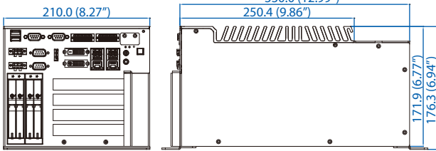
RCS-9000F GTX1080
